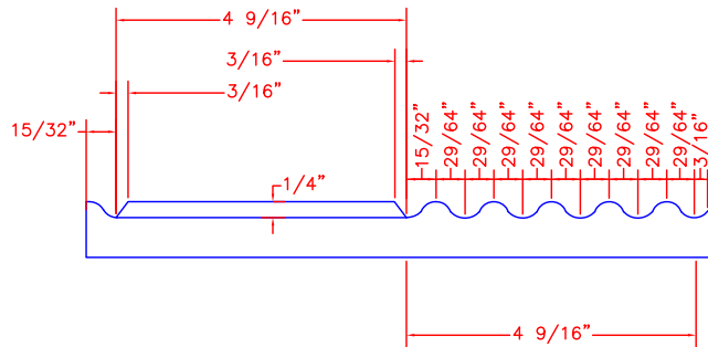
SURFACE DETAIL
