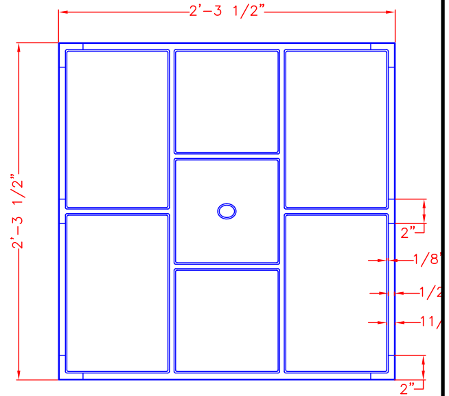
PLAN OF BOTTOM OF COVER
